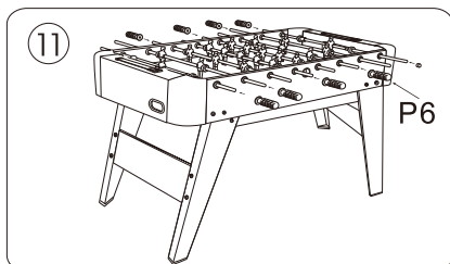
Insert 8 handles into the bars, make sure that all the handles are tightened.
